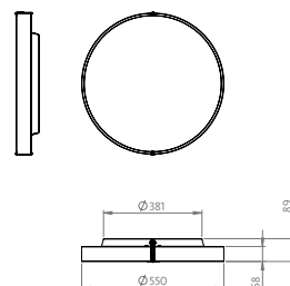
Ø550mm OP/MP
