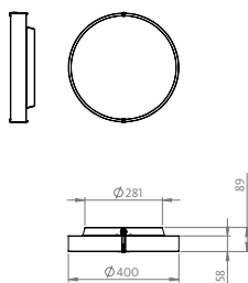
Ø400mm OP/MP
