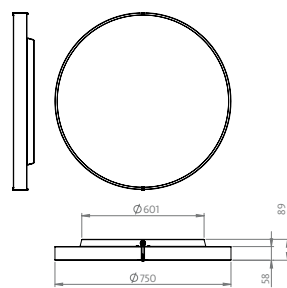
Ø750mm OP/MP
