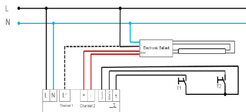
230V/AC
