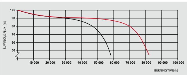
Service Life Aura ULTIMATE Signette Long Life - 3 h-switching cycle (2 h 45 min. on, 15 min. off)
